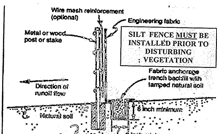
Figure 6.2-2: Typical Installation for Silt Fence
